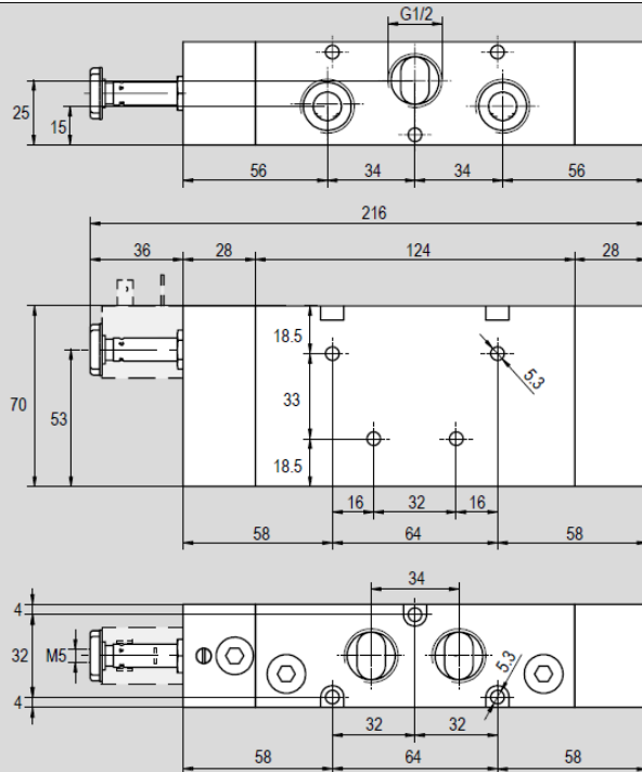
Type: 5/2 solenoid/spring with external air pilot
