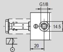
Type: 5/2 solenoid/spring with external air pilot
